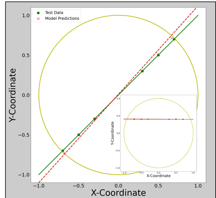
Validated Transits with Trained Model
